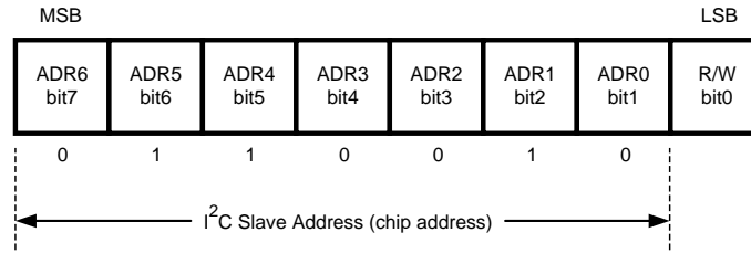
Figure 21. LP5523 Chip Address
