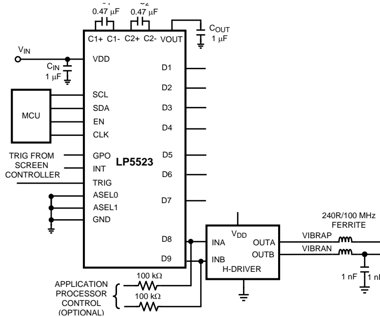
Figure 29. Example Schematic – Vibra Motor
