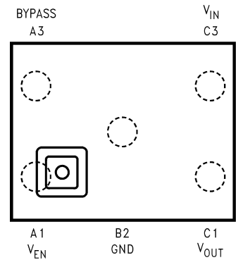
Top View See NS Package Number BPA05, BLA05, TLA05
