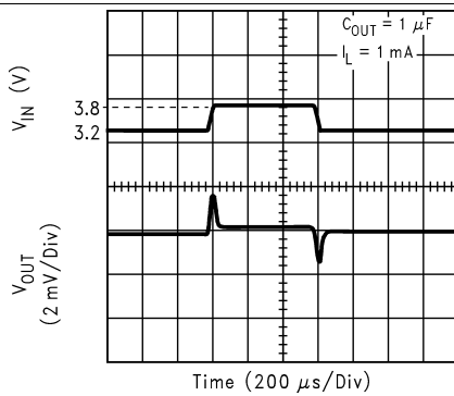
Figure 27. Line Transient Response
