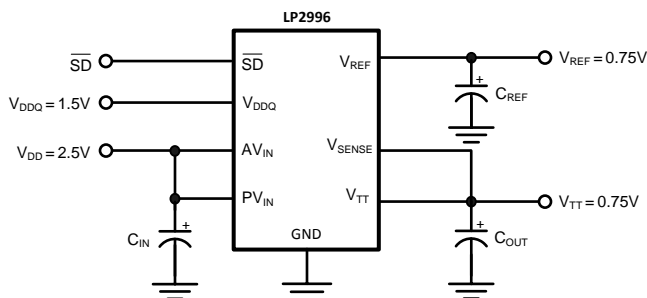
Figure 28. HSTL Application
