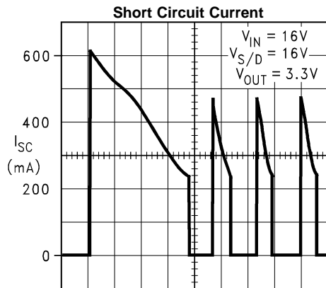
200 ms/Div Figure 19.
