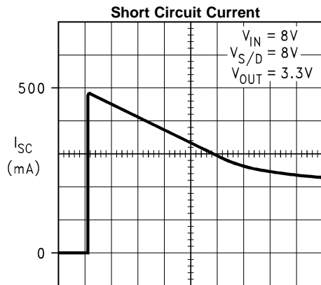
500 ms/Div Figure 18.
