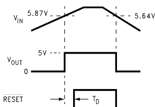
Figure 49. Timing Diagram
