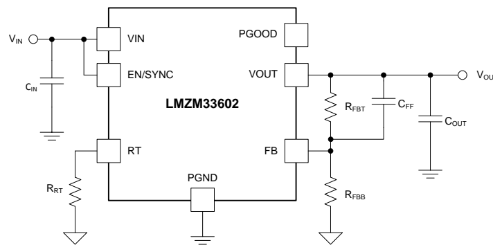
Figure 30. LMZM33602 Typical Schematic
