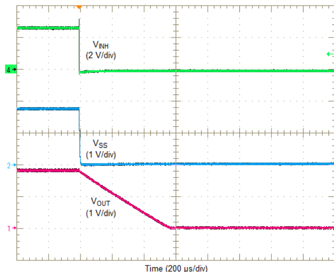
Figure 28. Inhibit Turn-Off
