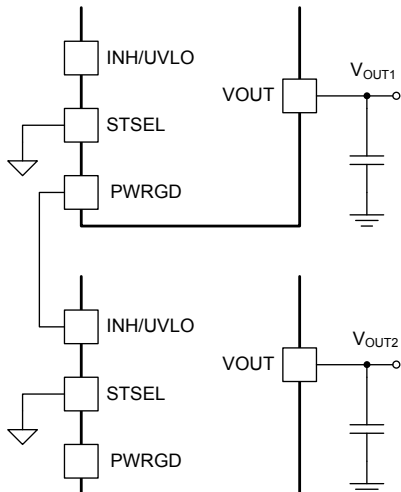
Figure 36. Sequencing Schematic
