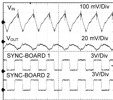
Figure 54. Output voltage ripple of two modules with synchronization clocks in phase
