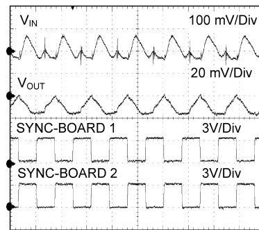
Figure 55. Output voltage ripple of two modules with synchronization clocks 180 degrees out of phase
