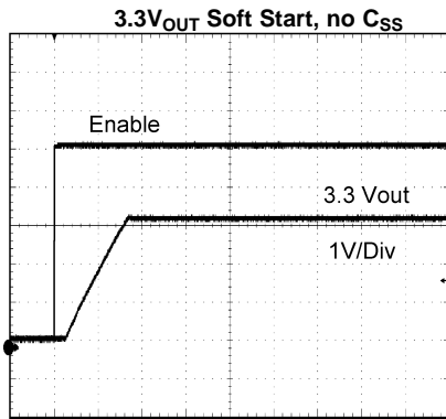
TIME (1 ms/Div) Figure 48.
