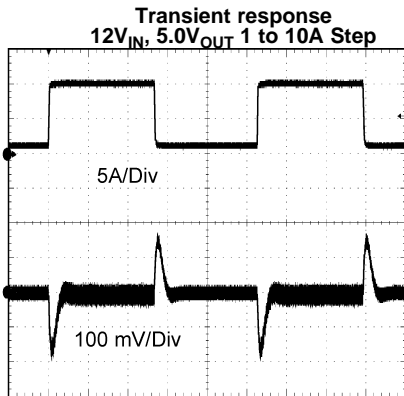
TIME (500 \mu s/Div) Figure 44.
