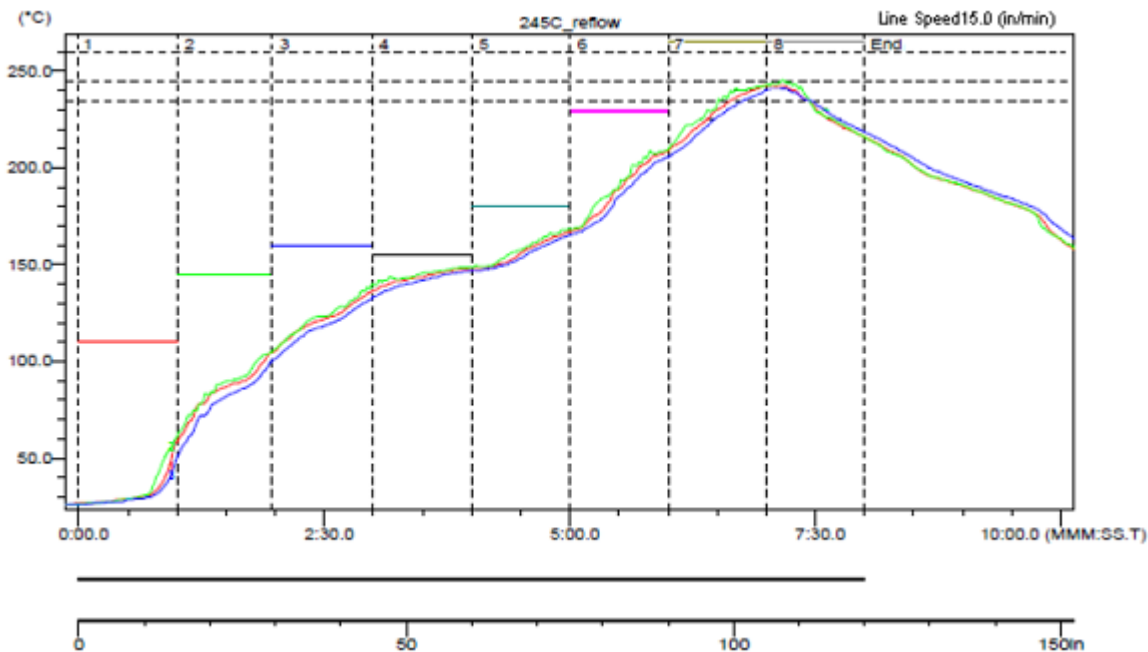
Figure 59. Sample Reflow Profile
