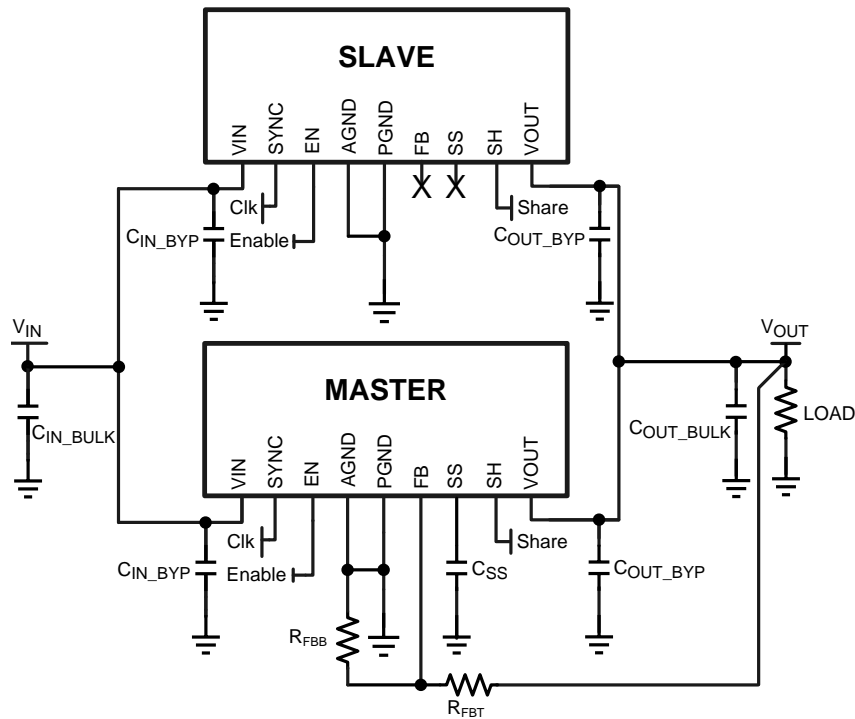
Figure 53. Current Sharing Example Schematic
