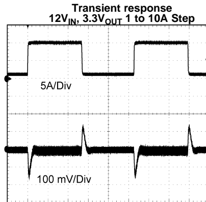
TIME (500 \mu s/Div) Figure 45.
