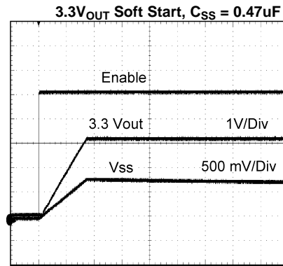
TIME (5 ms/Div) Figure 49.
