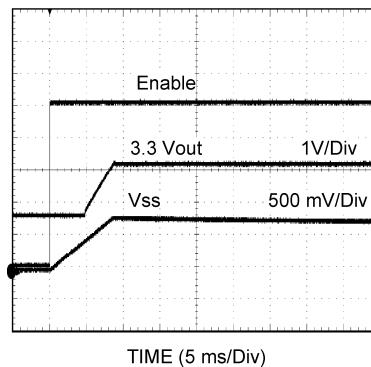
Figure 56. Pre-Biased Startup
