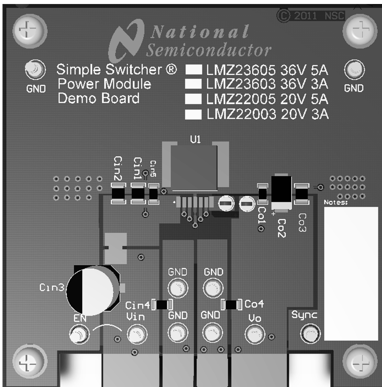
Figure 52. Top View Demonstration Board – See AN–2125 SNVA473
