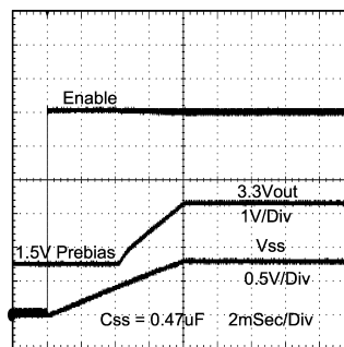
Figure 49. Pre-Biased Startup
