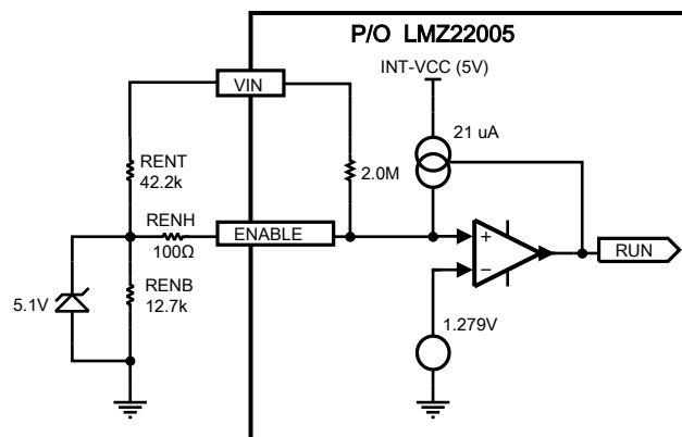
Figure 46. Enable Input Detail
