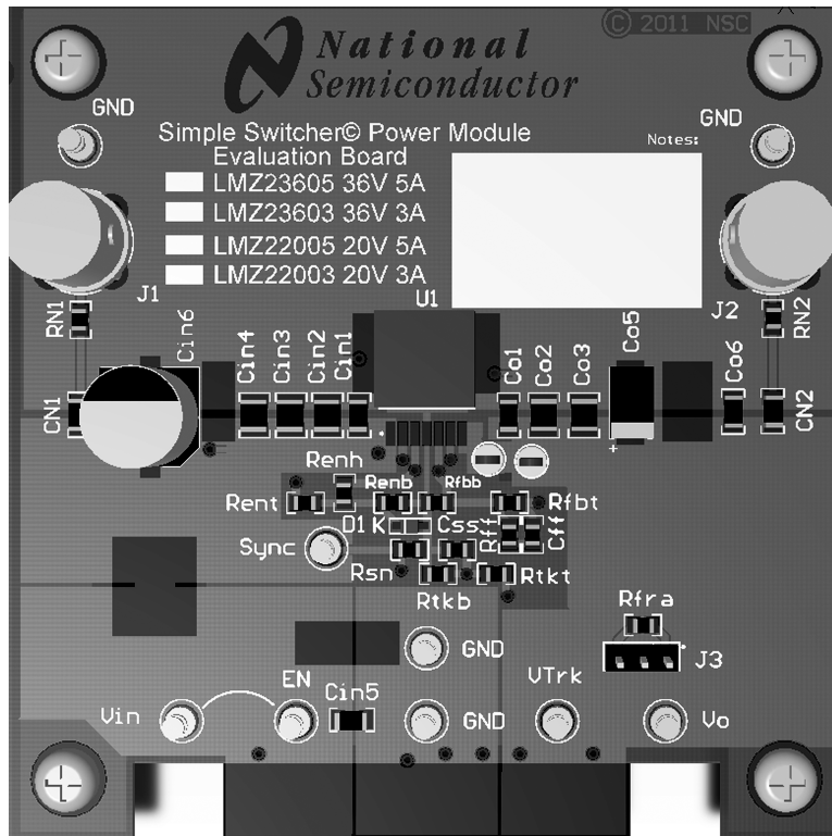
Figure 51. Top View Evaluation Board – See AN-2085 SNVA457
