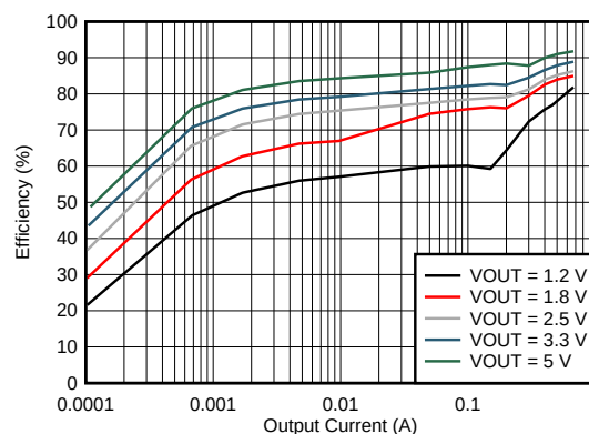
Efficiency for V_{IN} = 12\text{ V}
