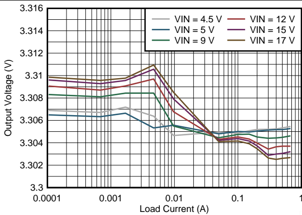
Figure 67. Line and Load Regulation V_{OUT} = 3.3\text{ V}
