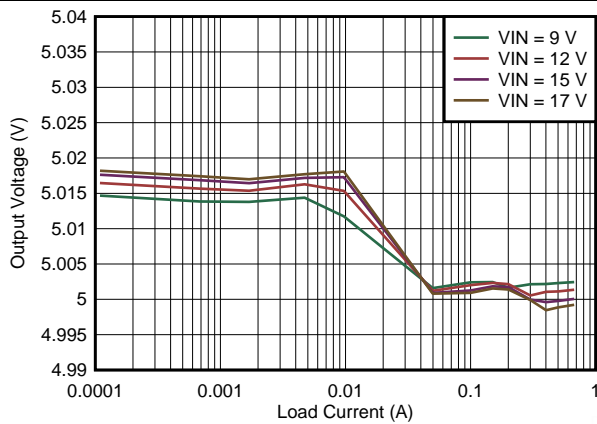
Figure 79. Line and Load Regulation V_{OUT} = 5.0\text{ V}
