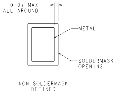
SOLDERMASK DETAILS NOT TO SCALE
