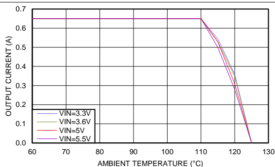
Figure 4. Thermal Derating V_{OUT} = 1.8\text{ V} , \theta_{JA} = 77^\circ\text{C/W}
