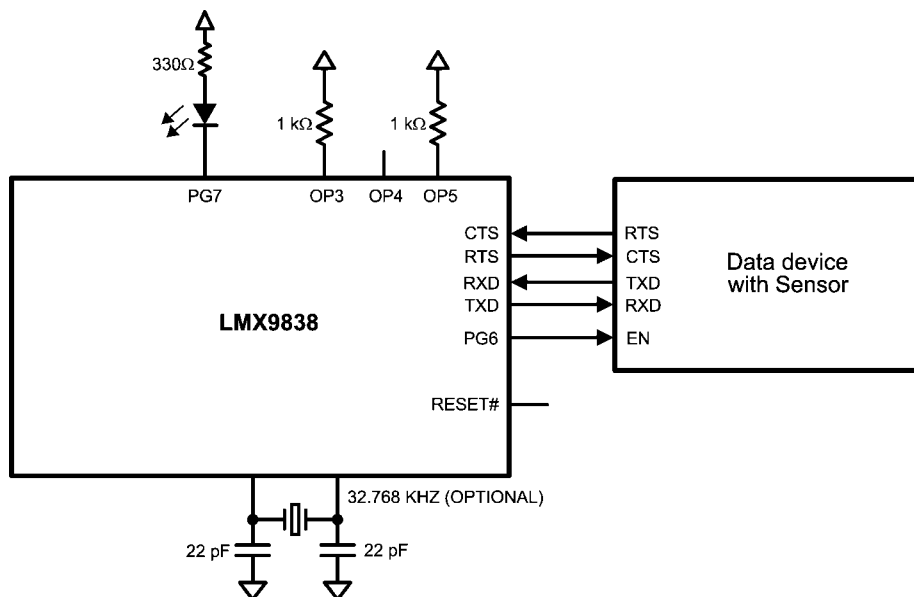
FIGURE 1. Example For A Cable Replacement Application
