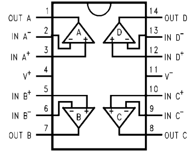
14-Pin TSSOP/SOIC (LMV934)
