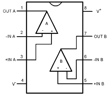
8-Pin MSOP/SOIC (LMV932)
