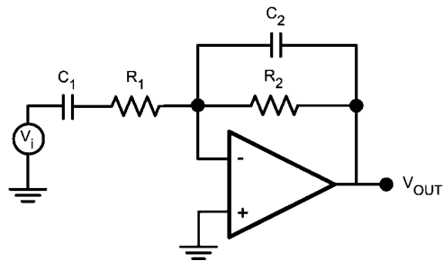
FIGURE 7. Bandpass Filter
