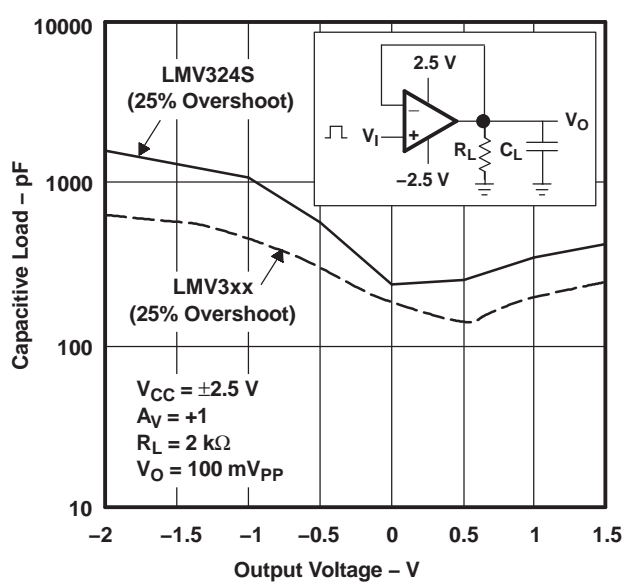
Figure 6. STABILITY VS CAPACITIVE LOAD
