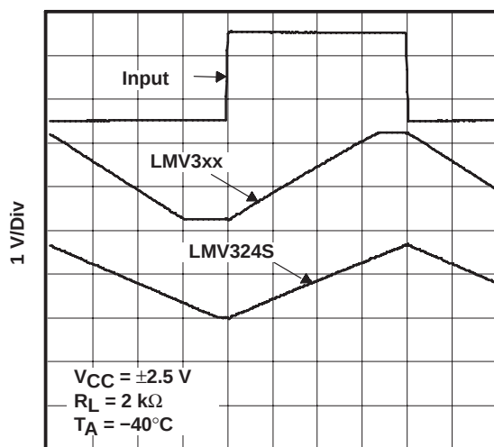
1 μs/Div Figure 29
