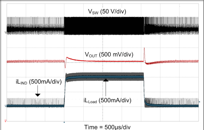
图 31. Load Transient (0 A - 1 A) at V_{IN} = 48\text{ V} at FPWM = 0
