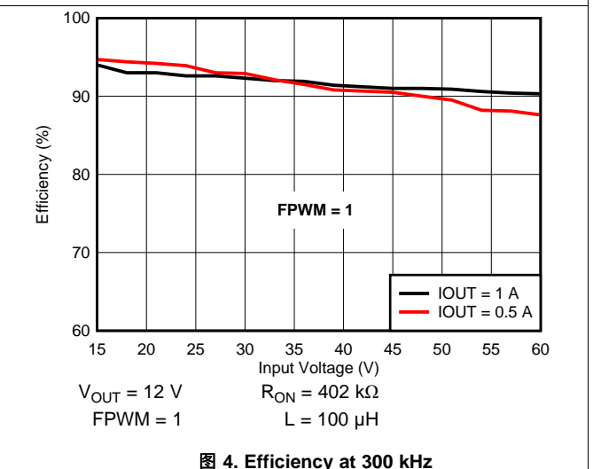
图 4. Efficiency at 300 kHz
