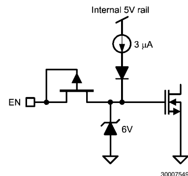
FIGURE 4. Enable Circuit
