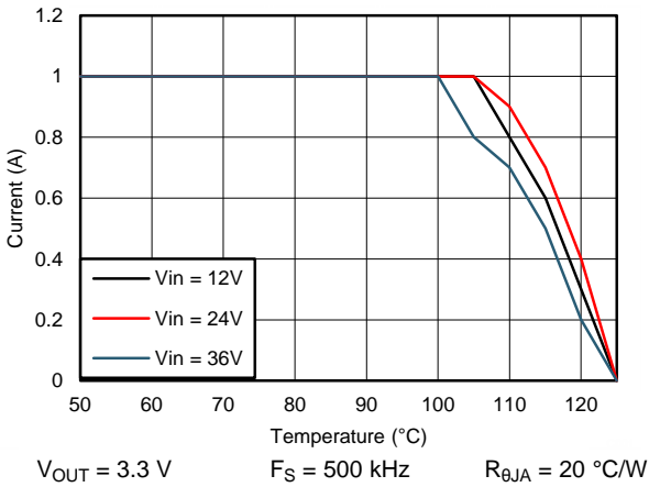
Figure 83. Derating Curve with R_{\theta JA} = 20\text{ }^\circ\text{C/W}
