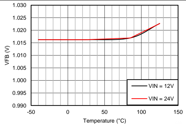
Figure 30. Feedback Voltage vs Junction Temperature
