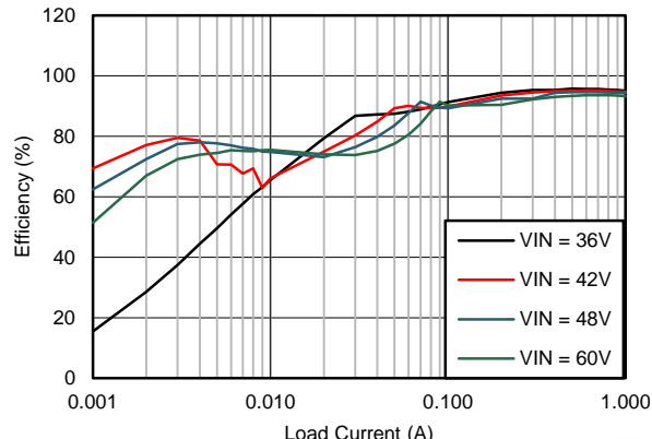
Figure 78. Efficiency
