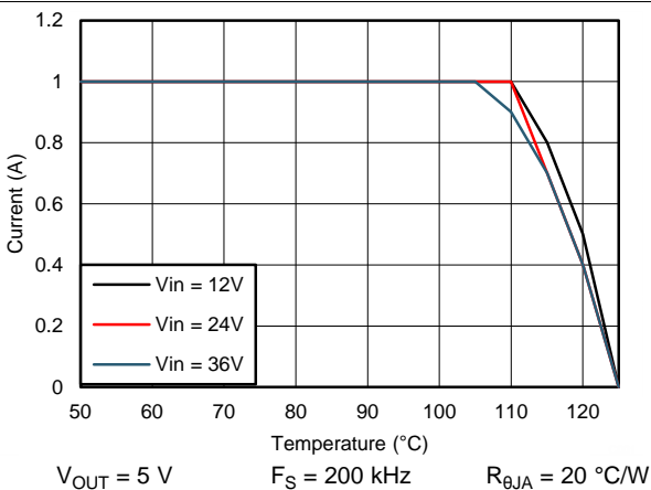
Figure 85. Derating Curve with R_{\theta JA} = 20\text{ }^\circ\text{C/W}
