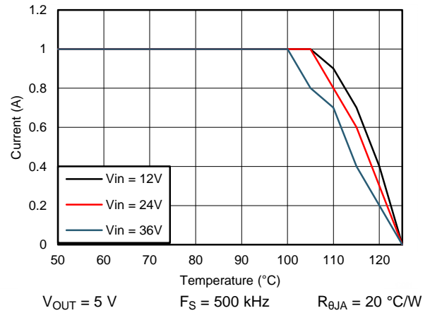
Figure 84. Derating Curve with R_{\theta JA} = 20\text{ }^\circ\text{C/W}
