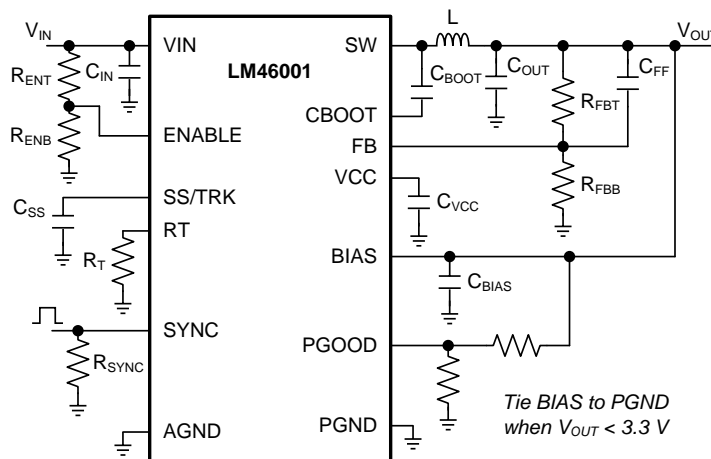
Figure 46. LM46001 Schematic with All Features
