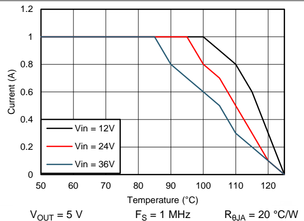
Figure 86. Derating Curve with R_{\theta JA} = 20\text{ }^\circ\text{C/W}
