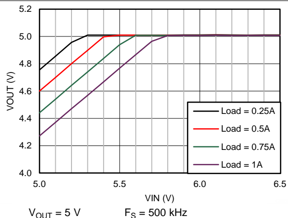
Figure 56. Drop-Out Curve
