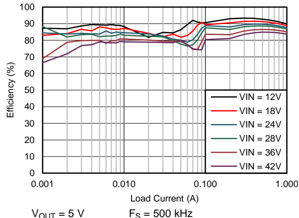
Figure 54. Efficiency
