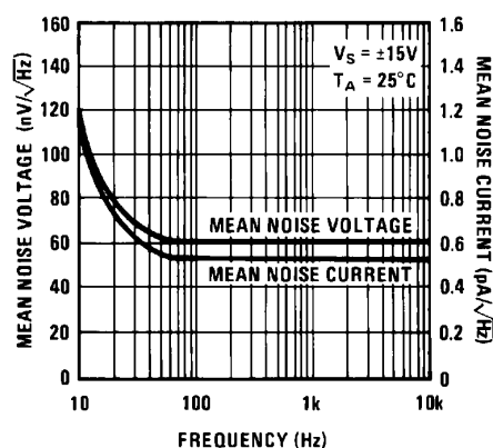
Input Noise Voltage and Noise Current
