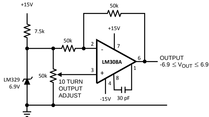
Figure 4. Adjustable Bipolar Output Reference
