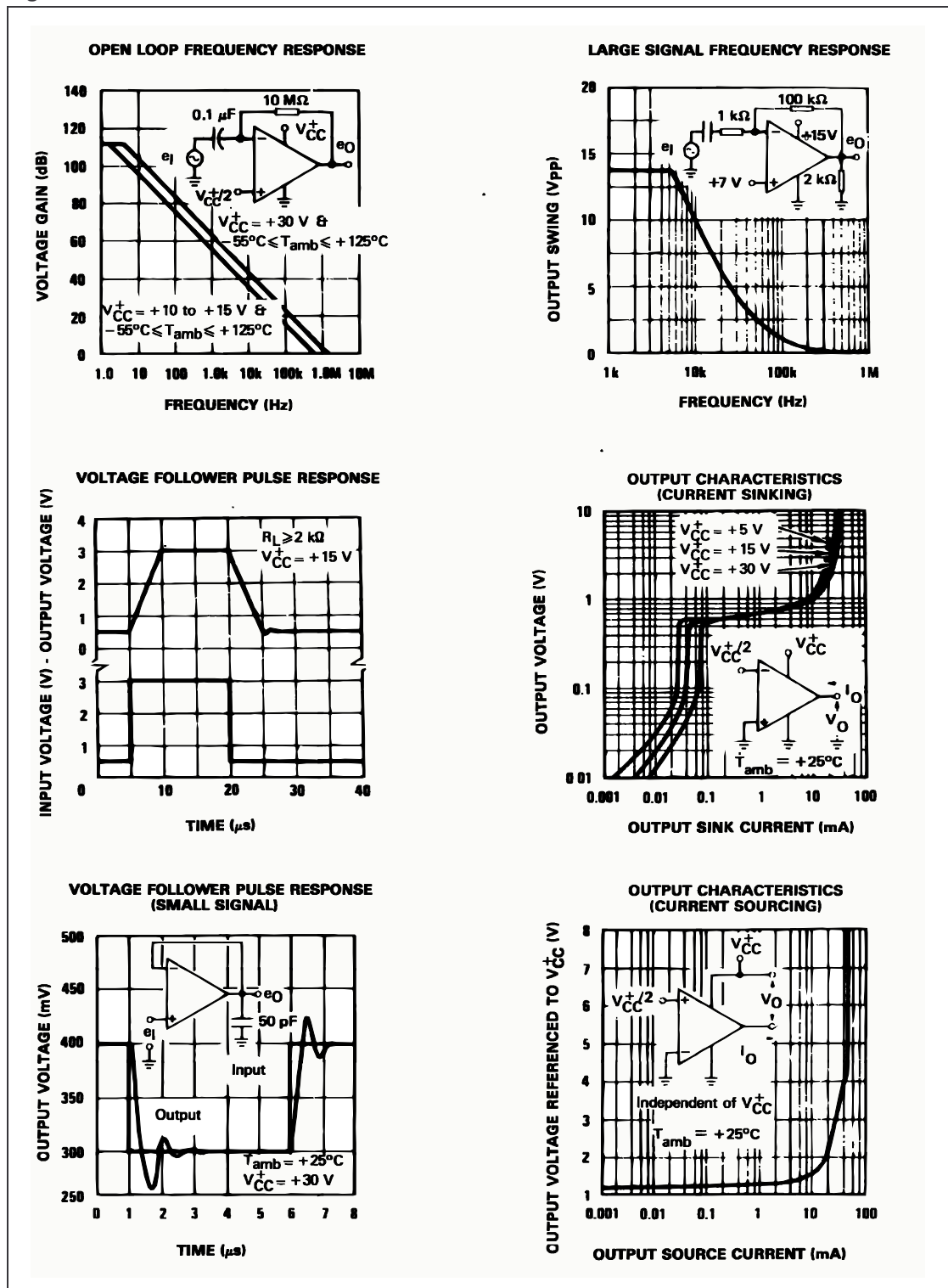
Figure 9. Electrical curves
