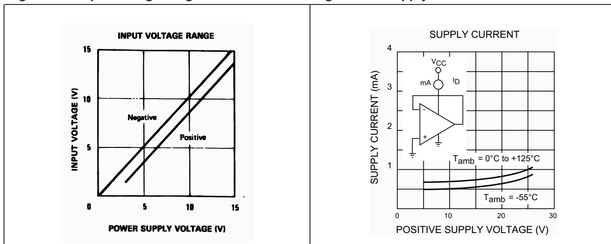
Figure 6. Supply current
