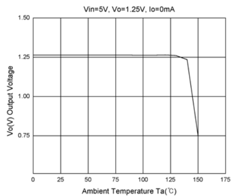
Figure 8. Thermal Shutdown
