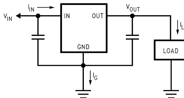
Figure 23. Power Dissipation Diagram
