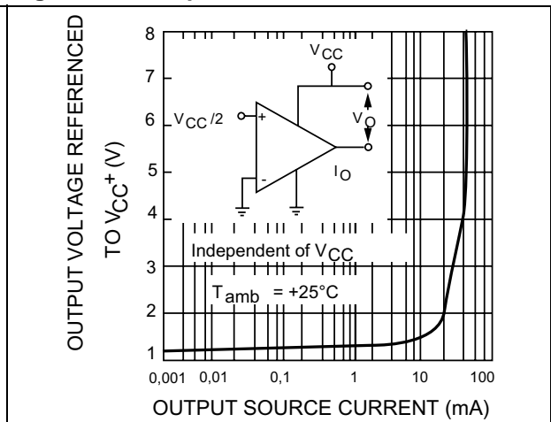
Figure 14. Output characteristics
