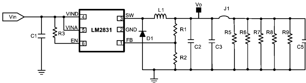
LM2831X 6-Pin LLP Demo Board Schematic
