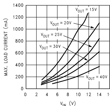
Figure 31. Max. Load Current vs VIN - "Y"
