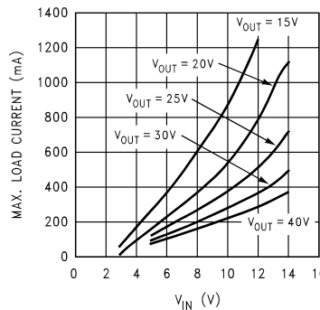
Figure 30. Max. Load Current vs VIN - "X"
