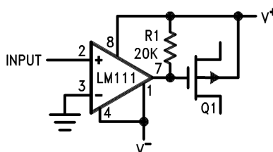
Figure 34. Zero Crossing Detector Driving MOS Switch
