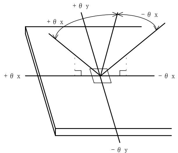
Fig.4 Definition of Viewing Angle
