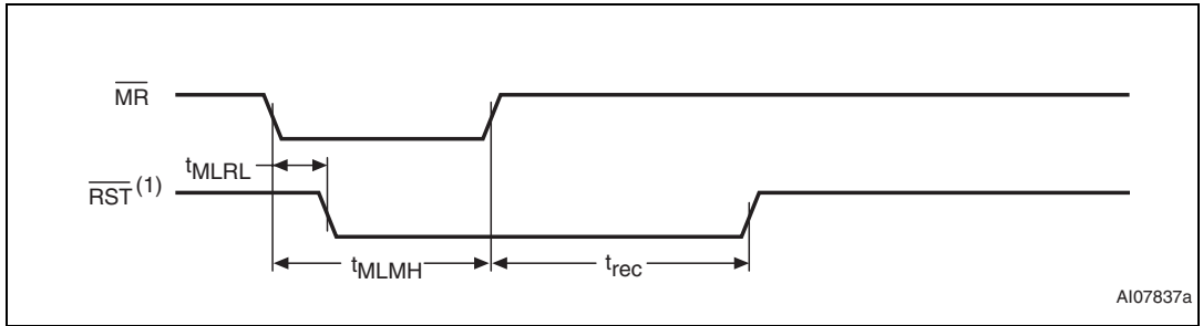
Figure 28. \overline{\text{MR}} timing waveform
