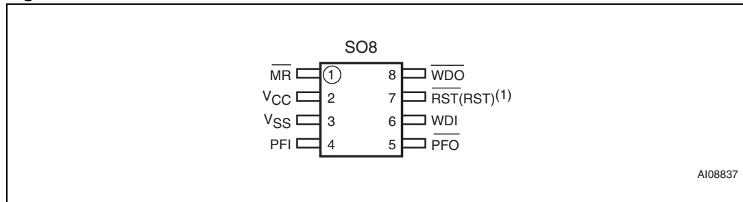
Figure 3. STM706T/S/R and STM706P SO8 connections
