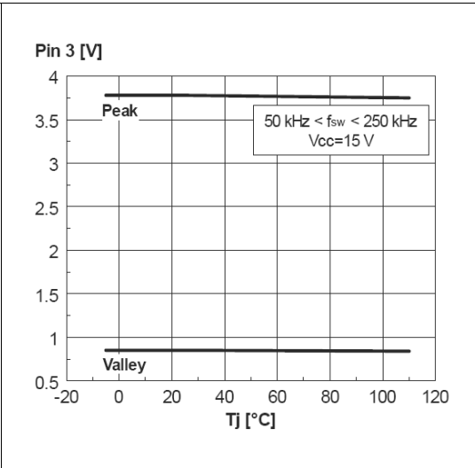
Figure 10. Oscillator ramp vs junction temperature
