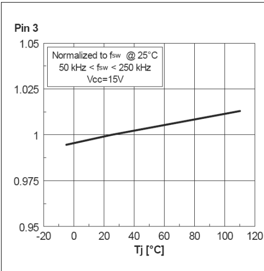
Figure 7. Oscillator frequency vs junction temperature
