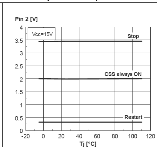
Figure 14. OCP delay thresholds vs junction temperature
