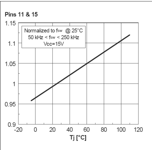
Figure 8. Dead-time vs junction temperature
