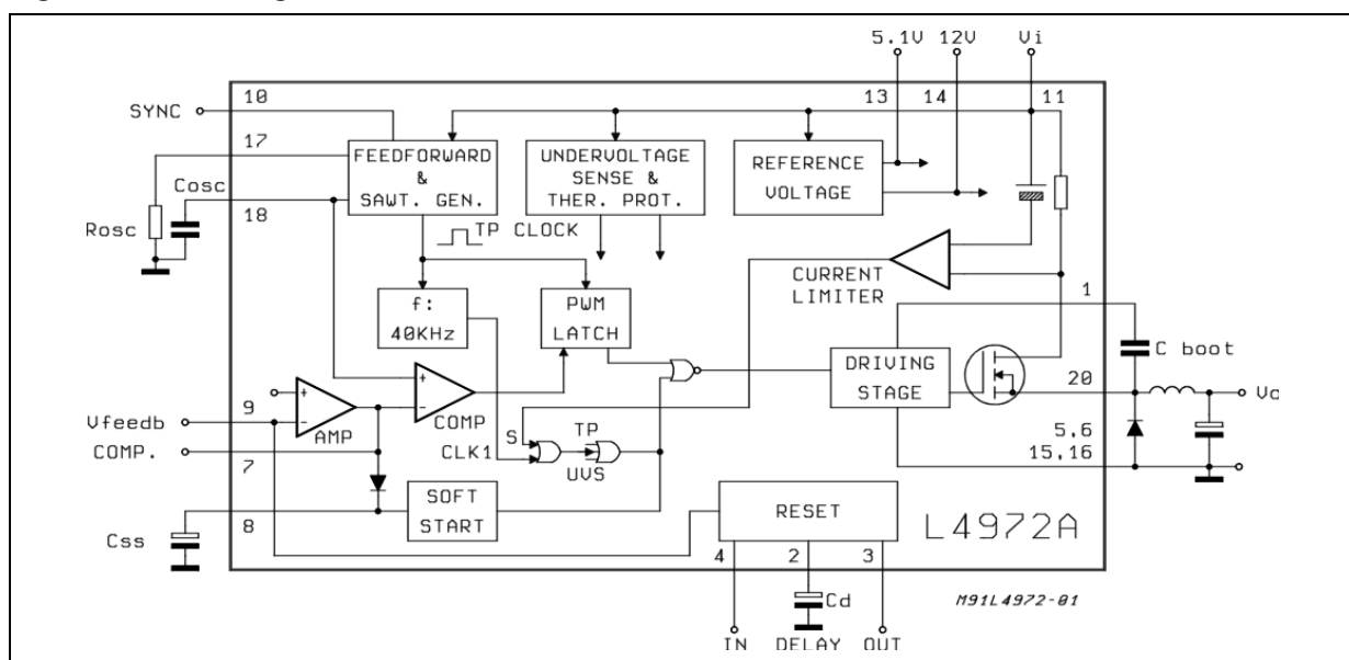
Figure 2. Block Diagram
