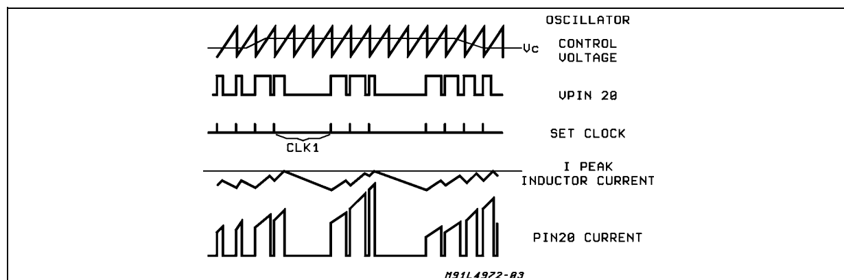
Figure 6. Limiting Current Function.
