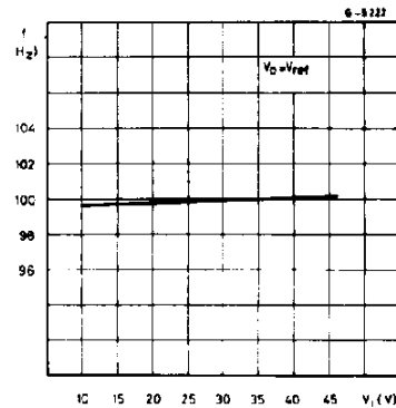
Figure 11. Switching frequency vs. input voltage
