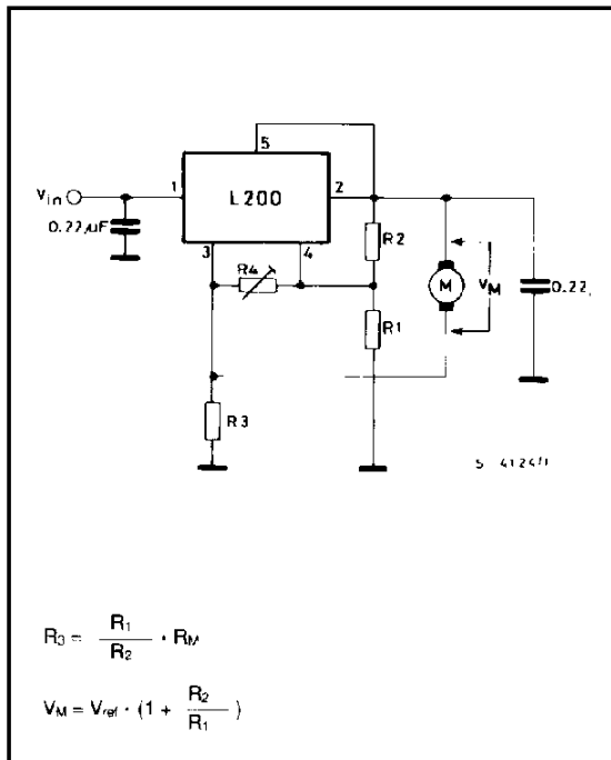
Figure 28. 30 W Motor Speed Control.
