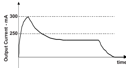
Figure 4. Driver Short-Circuit Test Circuit and Waveforms (Short Circuit applied at Time t=0 )
