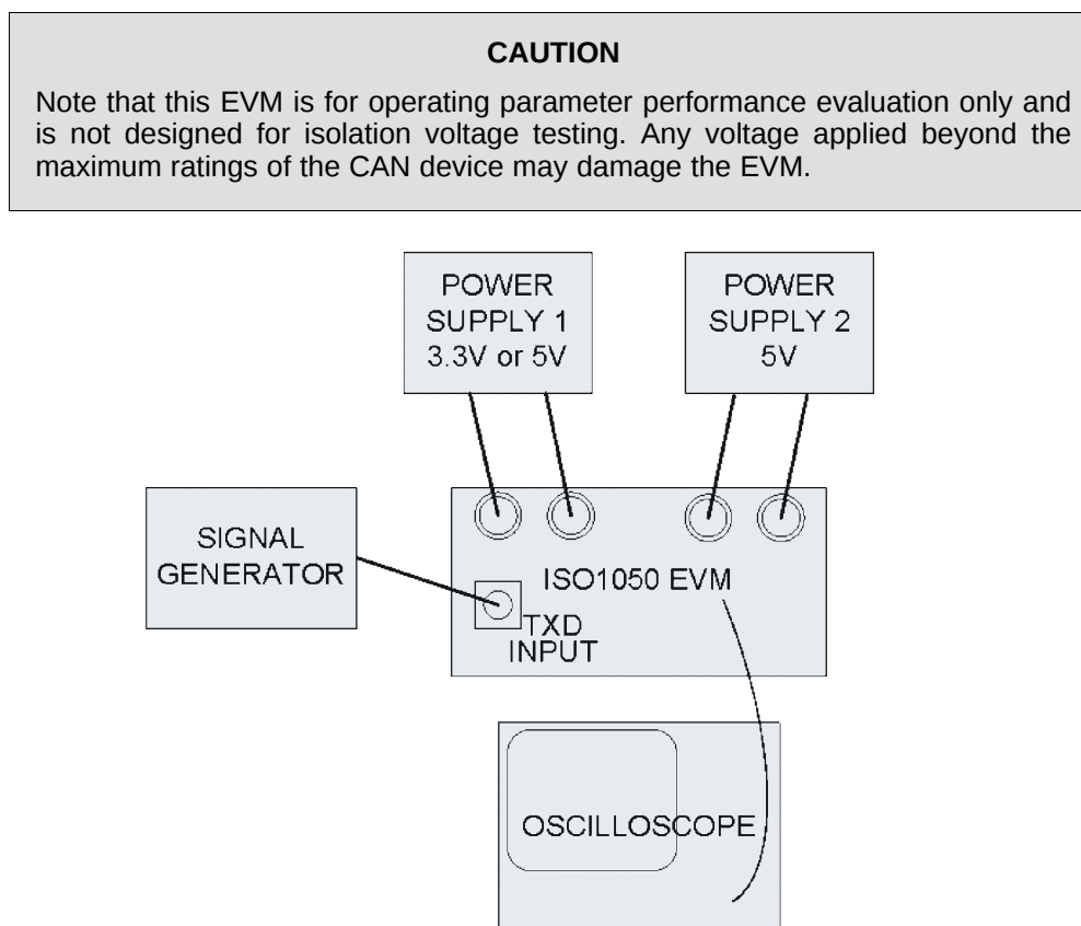
Figure 4. Basic Isolated CAN Transceiver EVM Operation
