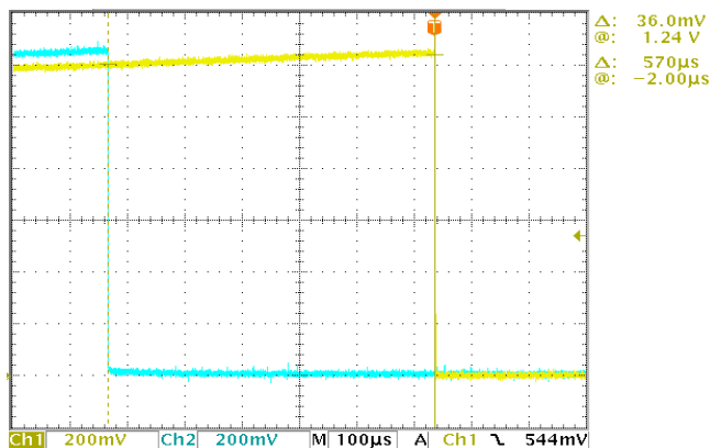
FIGURE 28. CAPACITOR TIMING MISMATCH
