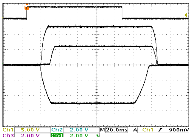
FIGURE 24. ±VOLTAGE SEQUENCING
