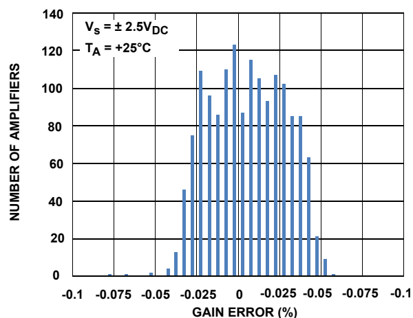
FIGURE 9. PGIA GAIN ERROR DISTRIBUTION, G = 1 \text{ TO } 1,000
