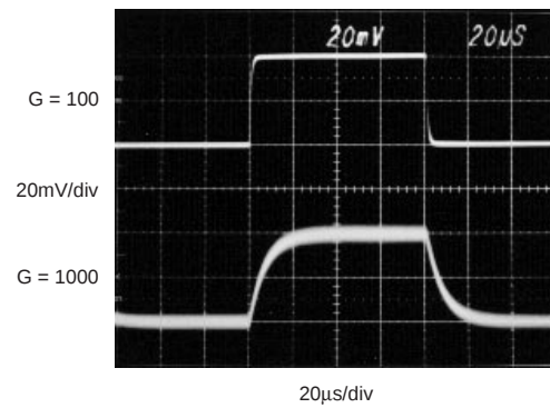
SMALL-SIGNAL STEP RESPONSE ( G = 100, 1000 )
