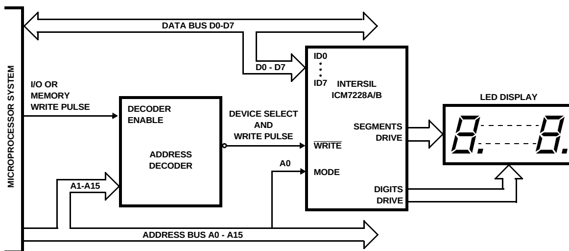
FIGURE 9. ICM7228A/B MICROPROCESSOR SYSTEM INTERFACING
