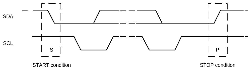
Figure 8. START and STOP Conditions
