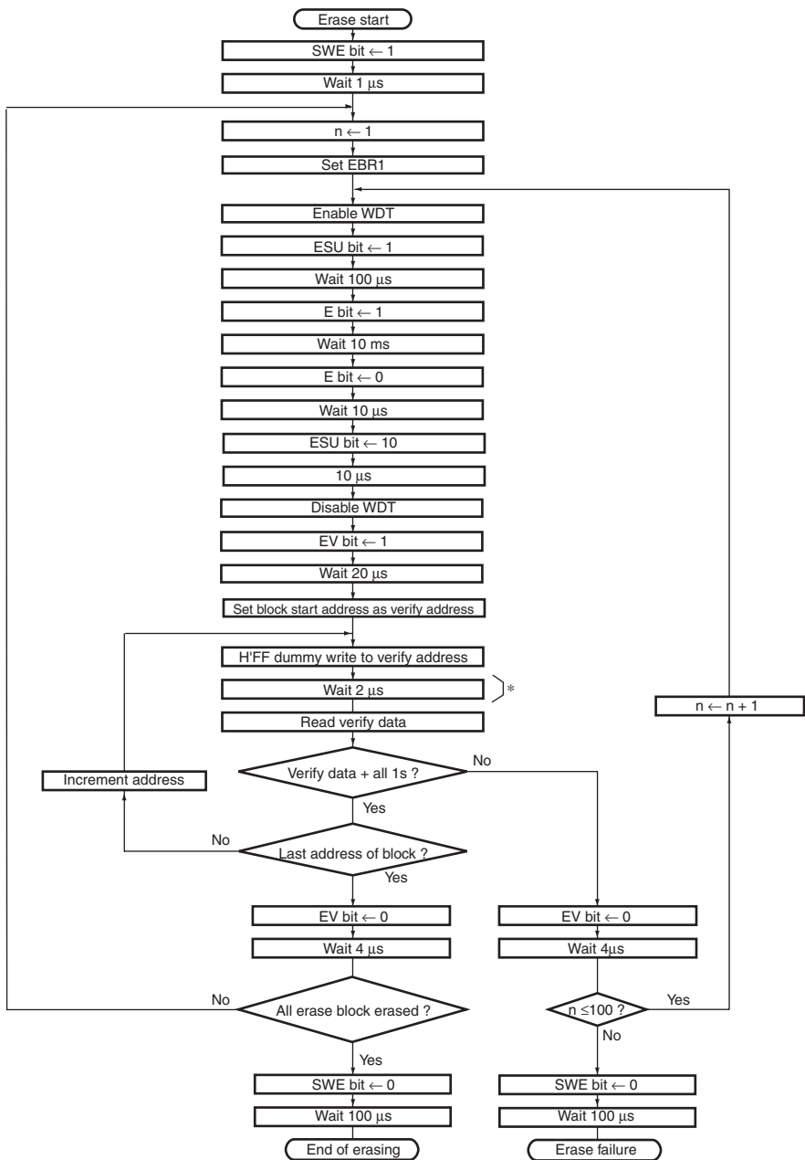
Figure 7.4 Erase/Eraser-Verify Flowchart
