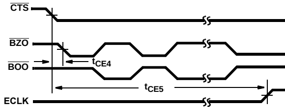
FIGURE 12. ENCODER TIMING
