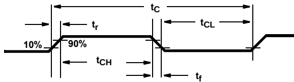
FIGURE 9. CLOCK TIMING
