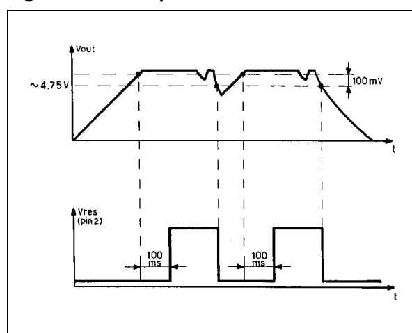
Figure 3. Reset Operation
