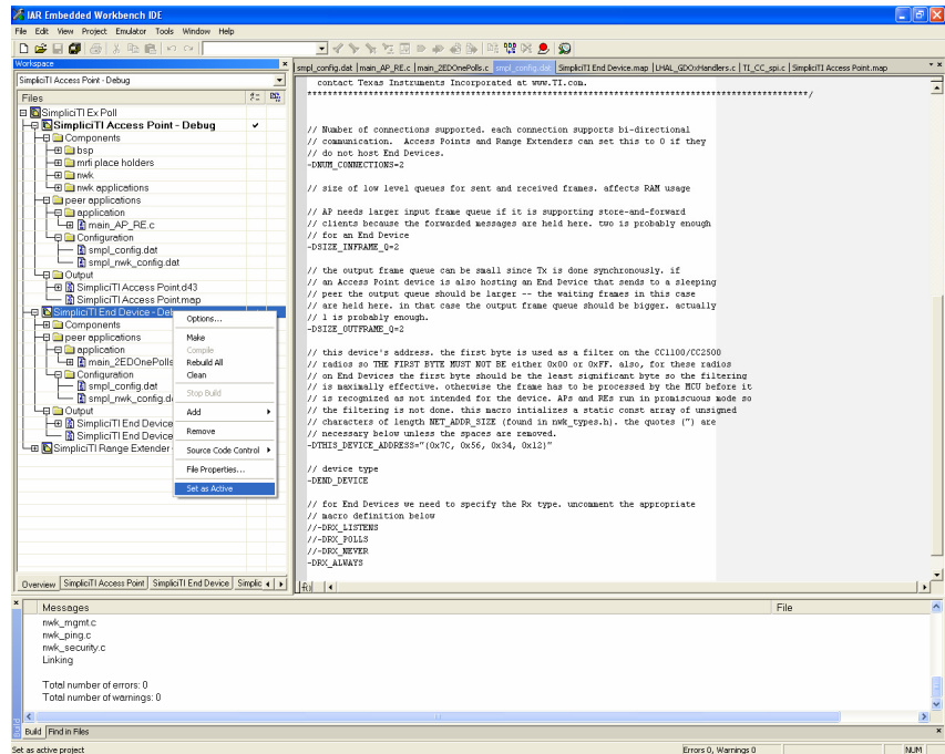
Figure 6. IAR Embedded Workbench Kickstart Workspace
