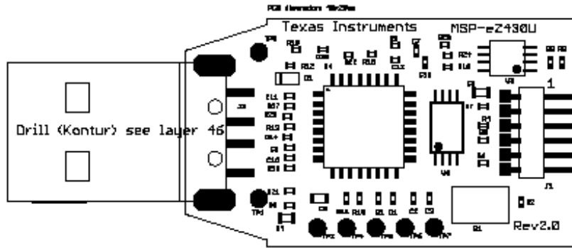
Figure 10. eZ430-RF, USB Debugger, PCB Components Layout
