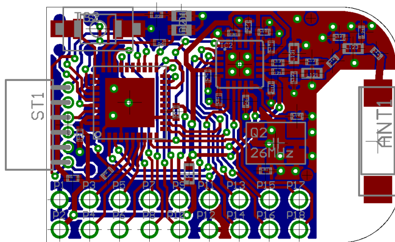
Figure 12. eZ430-RF2500T, Target Board, PCB Layout
