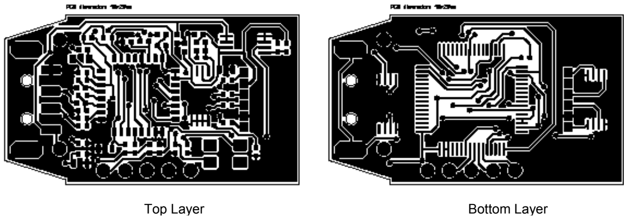
Figure 11. eZ430-RF, USB Debugger, PCB Layout
