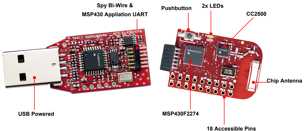
Figure 1. eZ430-RF2500
