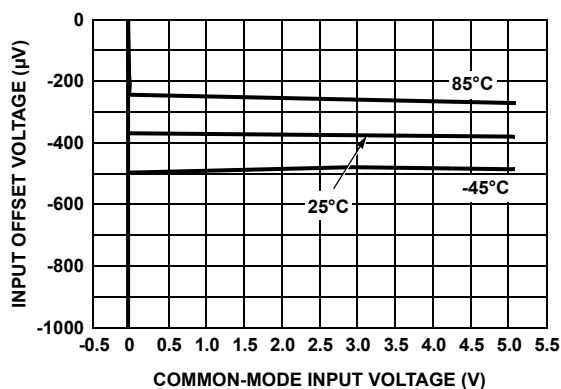
FIGURE 20. EL8173 INPUT OFFSET VOLTAGE vs COMMON-MODE INPUT VOLTAGE @ V_S = 5.0V , TEMPERATURE = -45°C, 25°C, AND 85°C
