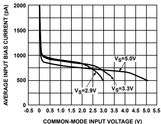
FIGURE 8. EL8173 AVERAGE INPUT BIAS CURRENT vs COMMON-MODE INPUT VOLTAGE @ 25°C
