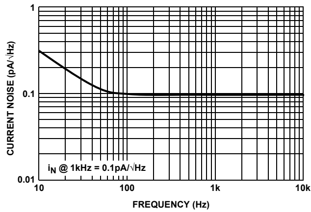
FIGURE 35. EL8170 AND EL8173 CURRENT NOISE DENSITY
