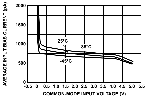
FIGURE 12. EL8173 AVERAGE INPUT BIAS CURRENT vs COMMON-MODE INPUT VOLTAGE @ V_S = 5V , TEMPERATURE = -45°C, 25°C, AND 85°C
