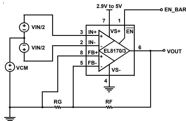
FIGURE 41. GAIN IS SET BY TWO EXTERNAL RESISTORS, RF AND RG
