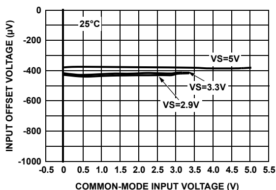
FIGURE 18. EL8173 INPUT OFFSET VOLTAGE vs COMMON-MODE INPUT VOLTAGE @ V_S = 5V , 3.3V, AND 2.9V AND TEMPERATURE = 25°C
