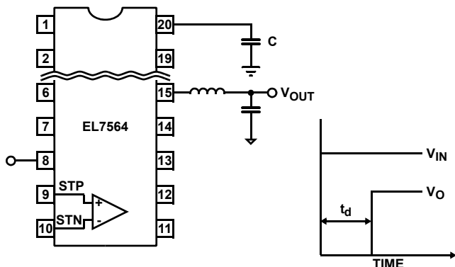
FIGURE 28. START-UP DELAY
